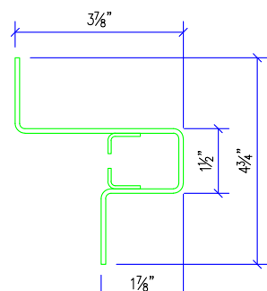
M4000 SIDE GUIDE
