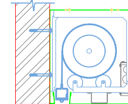
M2500 LARGE HOUSING FOR 12' AND OVER CLEAR OPENING HEIGHT
