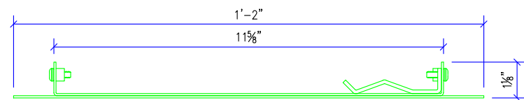
M4000 CURTAIN TRAY W/OPTIONAL 14" FINISH COVER
