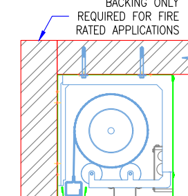
M2500 LARGE HOUSING FOR 12' AND OVER CLEAR OPENING HEIGHT
