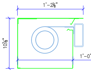
M3000 HEAD BOX HOUSING
