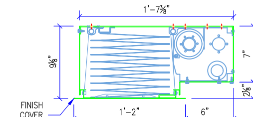
M4000 HOUSING
