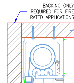
M2500 SMALL HOUSING FOR UNDER 12' CLEAR OPENING HEIGHT
