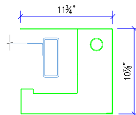
M3000 FOOT BOX HOUSING
