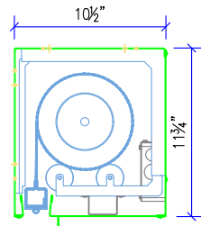
M2500 LARGE HOUSING FOR 12' AND OVER CLEAR OPENING HEIGHT
