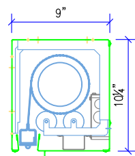
M2500 SMALL HOUSING FOR UNDER 12' CLEAR OPENING HEIGHT
