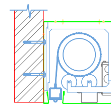
M2500 SMALL HOUSING FOR UNDER 12' CLEAR OPENING HEIGHT
