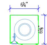
M2100 HOUSING
